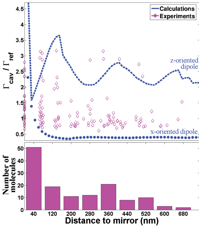
FIG. 12. (Color online) Distribution of the fluorescence decay rate as a function of distance to the closest Bragg mirror for all cavity sizes (purple diamonds). The dotted (dashed) curve is the minimum (maximum) calculated decay rate for an x -oriented ( z -oriented) dipole.
