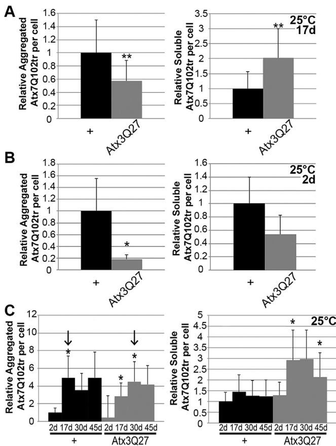
Fig. 3. Effects of Atx3Q27 and aging on Atx7Q102tr protein levels. Relative Atx7Q102tr cellular levels measured in flies raised at 25 °C in the absence (black) or presence of Atx3Q27 (grey). Flies were 17- (A), 2- (B) or 2-, 17-, 30- or 45-day-old (C). The relative aggregated Atx7Q102tr level (left histograms) is the ratio between the dot blot signal and the glass signal. The relative soluble Atx7Q102tr level (right histograms) is the ratio between the western blot signal and the glass signal. (A, B) Statistical difference with the first condition on the histogram is indicated by * when p < 5\% and ** when p < 1\% (ANOVA). (C) Statistical difference with the preceding time is indicated by * (ANOVA, p < 5\% ). Arrows indicate the onset of eye degeneration revealed by the loss of pigment cells. Genotypes: GMR-gal4/+;UAS-atx7Q102tr/+ (+), GMR-gal4/UAS-atx3-Q27;UAS-atx7Q102tr/+ (Atx3Q27).
