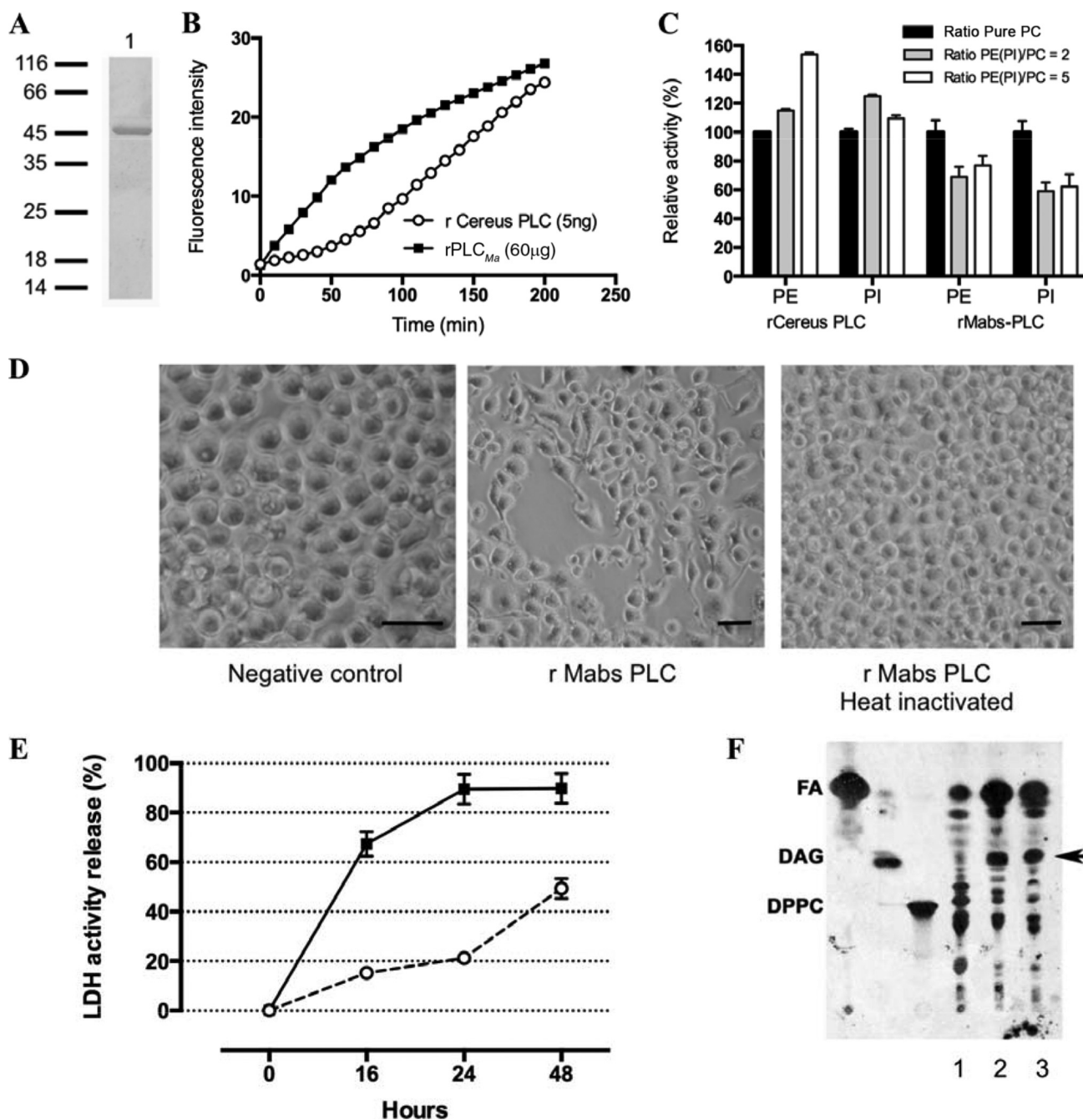
FIG 1 (A, B, and C) Biochemical characterization of rPLC Ma . (A) Purified rPLC Ma was loaded on 12% SDS-PAGE. Molecular weight standards are on the left. Lane 1 contained purified rPLC Ma (10 μg). The sample was loaded under reducing conditions, and the gel was then stained with Coomassie brilliant blue. (B) Time course hydrolysis of phosphatidylcholine (PC) by 60 μg of rPLC Ma (■) or 5 ng of recombinant B. cereus PC-PLC (○). The release of phosphocholine was measured indirectly by the fluorescence measurement of resorufin released using the Amplex red phosphatidylcholine kit and continuously monitored at a \lambda_{exc} of 510 nm and \lambda_{em} of 590 nm. (C) Substrate preference of rPLC Ma and recombinant B. cereus PC-PLC. Competition assays between PC and phosphatidylethanolamine (PE) (or phosphatidylinositol [PI]) were carried out using different phospholipid ratios (PE [or PI]/PC = 2 or 5) and pure PC. A final PC quantity of 0.1 μmol was used in the pure-PC assay, and 0.2 μmol and 0.5 μmol of PE (or PI) were used for the other PE (PI)/PC ratios. The PC-PLC activity was continuously measured using the Amplex red PC-PLC kit. The relative activity (percent) of PC hydrolysis was calculated from the ratio of PC activity in the presence of PE (or PI) over PC activity in the absence of PE (or PI). (D, E, and F) Cytotoxic effects of rPLC Ma on mouse macrophages. (D) Macrophage cellular state after 24 h of incubation, with no recombinant PLC (buffer only [negative control]), with 50 μg of purified rPLC Ma (rPLC Ma ), and with 50 μg of heat-inactivated purified rPLC Ma (rPLC Ma , heat inactivated), as shown by light microscopy (magnification, \times 200 ; bar, 25 μm). (E) Purified rPLC Ma (50 μg; ■) and 15 μg of PC-PLC from B. cereus (○) were incubated with 1 \times 10^6 RAW264.7 mouse macrophages. The values are shown as percent lysis, in which the amount of LDH released in wells with macrophages incubated with enzymes was compared to total LDH released in control wells in which all of the macrophages had been deliberately lysed. LDH released was quantified at 16, 24, and 48 h. The values are the means for triplicate samples. (F) Autoradiography of TLC plate showing the release of radiolabeled DAG, the product of phospholipid hydrolysis (indicated by the black arrow), after incubation of rPLC Ma (50 μg, lane 2) and PC-PLC from B. cereus (15 μg, lane 3) with radiolabeled macrophages. For the negative control (lane 1), only the buffer without any pure enzyme was added in the incubation medium. Abbreviations: DAG, diacylglycerol; FA, free fatty acid; DPPC, dipalmitoyl-glycerophosphocholine.
