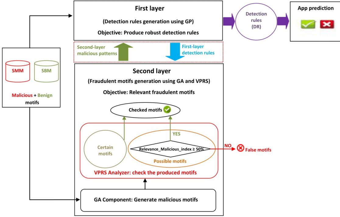
Fig. 2. Illustration of the ProRSDet functioning process.
