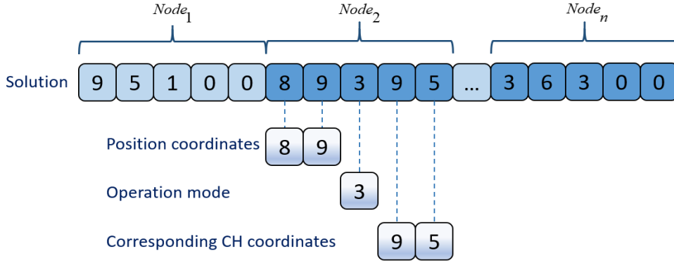
Fig. 2 Solution encoding
