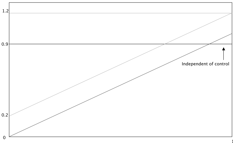
Figure 3.1 Transport equation
