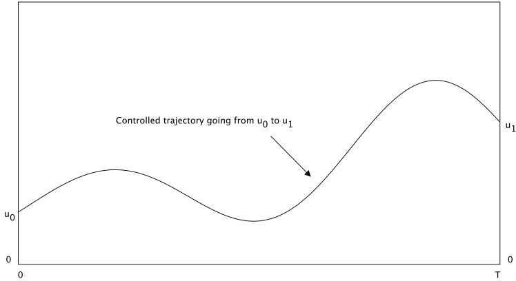
Figure 2.1 Exact controllability
