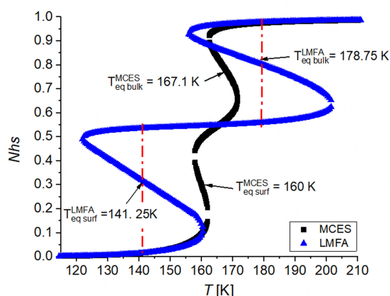
Figure 9. Comparison of the thermal evolution of the HS fraction in a SCO system for a 6 \times 6 square lattice: MCES (black squares), LMFA (blue up triangles). The computational parameters are: J_{bb}^{MCES}/k_B = 60 K, J_{ss}^{MCES}/k_B = 60 K, J_{bs}^{MCES}/k_B = 60 K, J_{bb}^{LMFA}/k_B = 60 K, J_{ss}^{LMFA}/k_B = 60 K, \Delta/k_B = 1,300 K, G/k_B = 172 K, L/k_B = 290 K, and \ln(g) = 6.01 .
